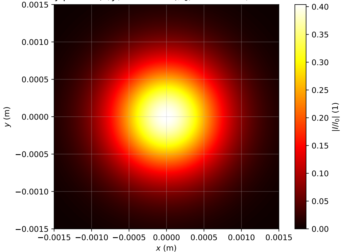
Intensity profile I(x, y, z = 3.901m)/I_0 , P_{in}=0.5P_{cr} , artificial time
